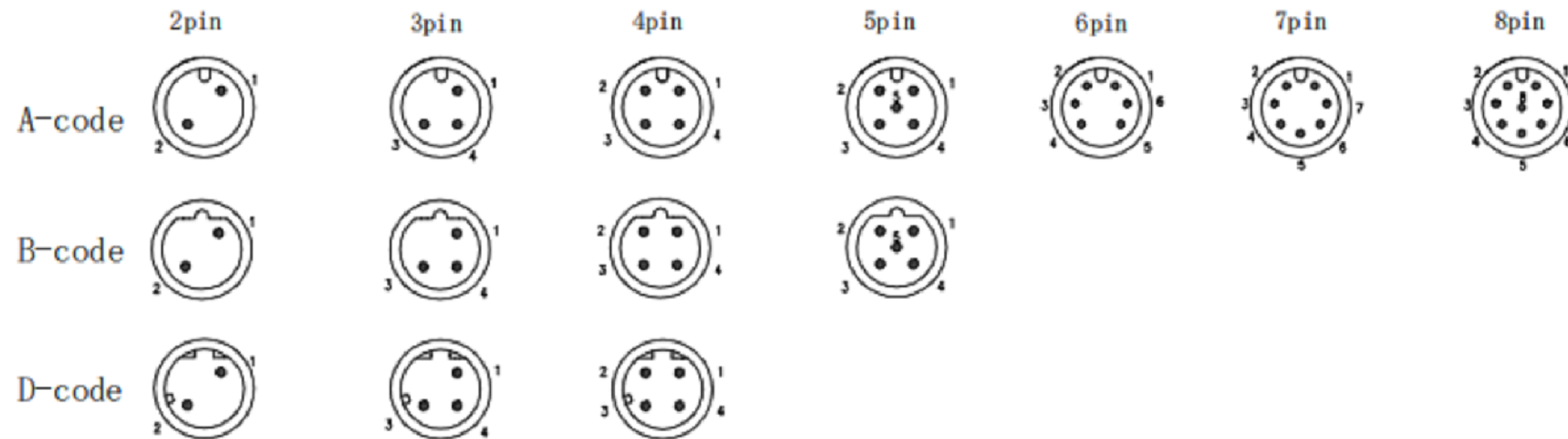
Pin assignment front view/针位分布前视图
